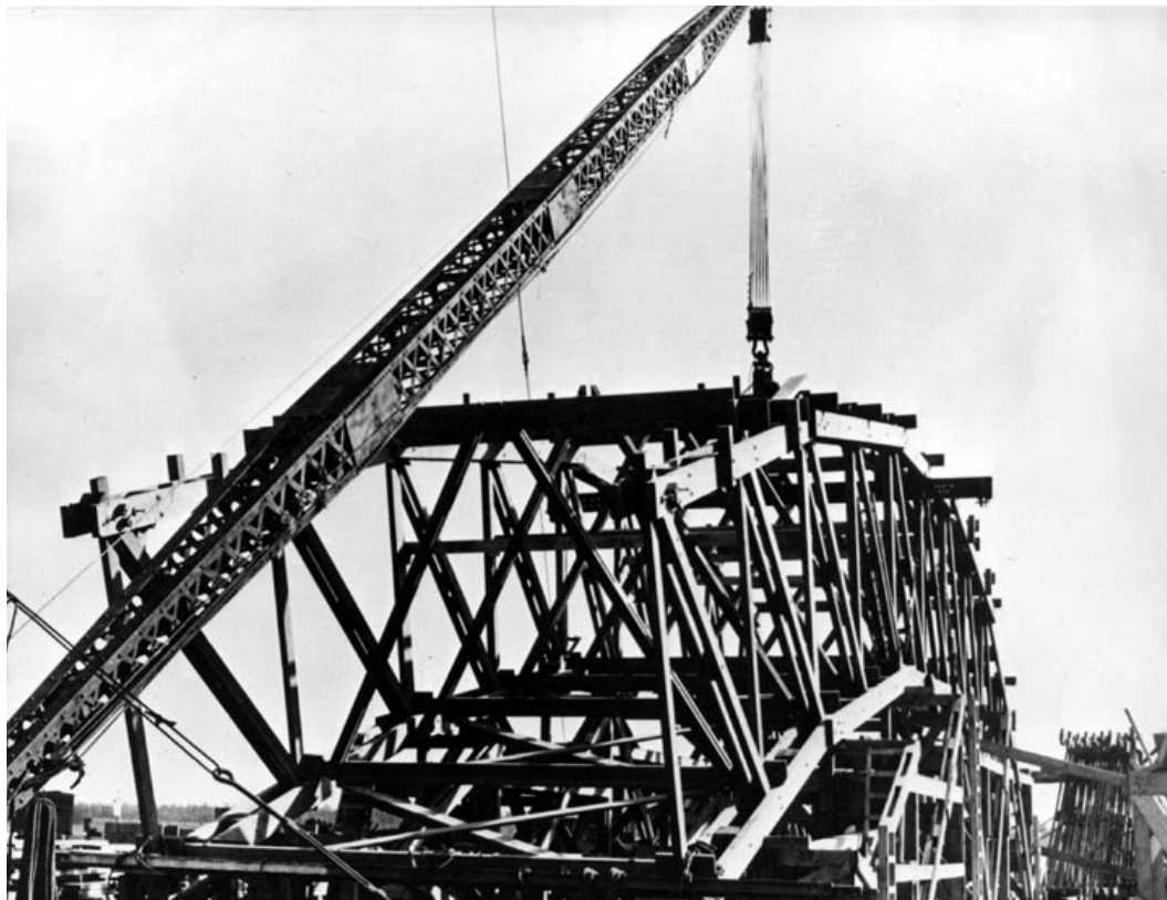
Hangar roof truss being set in place, 1943
